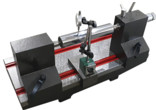
SLIDING ATTACHMENT FOR STRAIGHTNESS AND RUNOUT CHECKING
